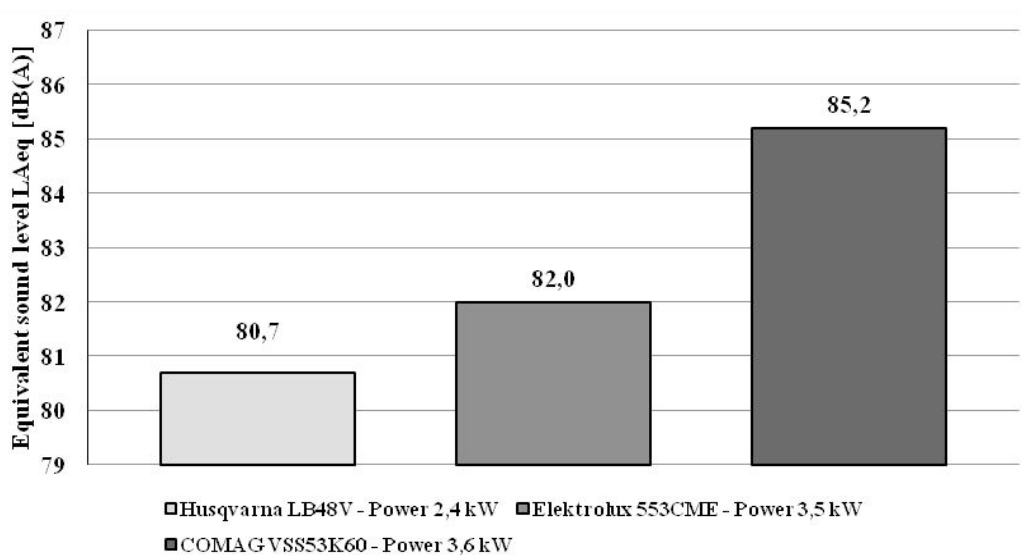
Fig. 6. The influence of engine power with the capacity of 190 – 198 cm 3 on the equivalent sound level L_{Aeq}
