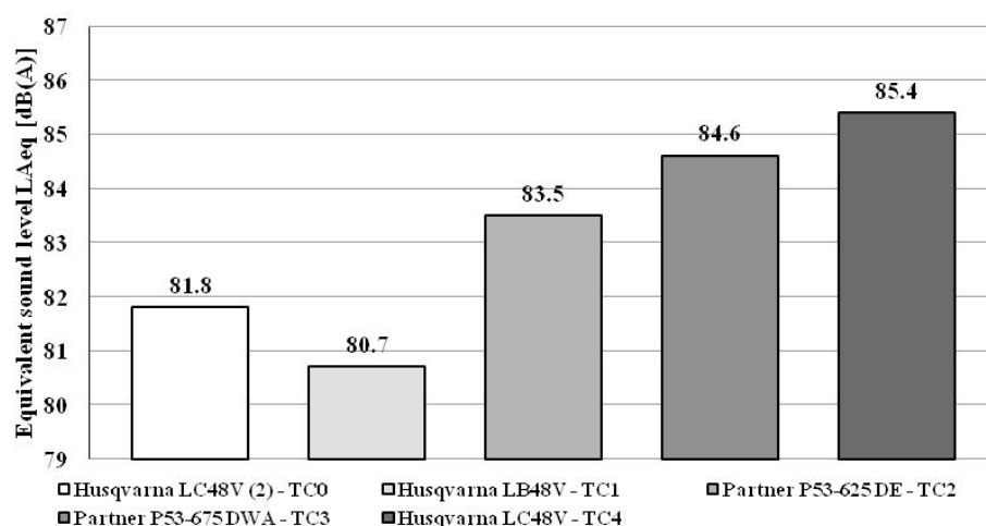
Fig. 3. The influence of the engine technical condition of the lawnmowers with the power – 2,4 kW and capacity – 190 cm 3 on the equivalent sound level L_{Aeq}
