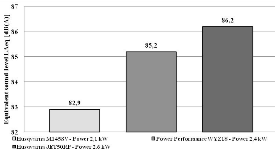
Fig. 5. The influence of engine power with the capacity of 148 – 158 cm 3 on the equivalent sound level L_{Aeq}
