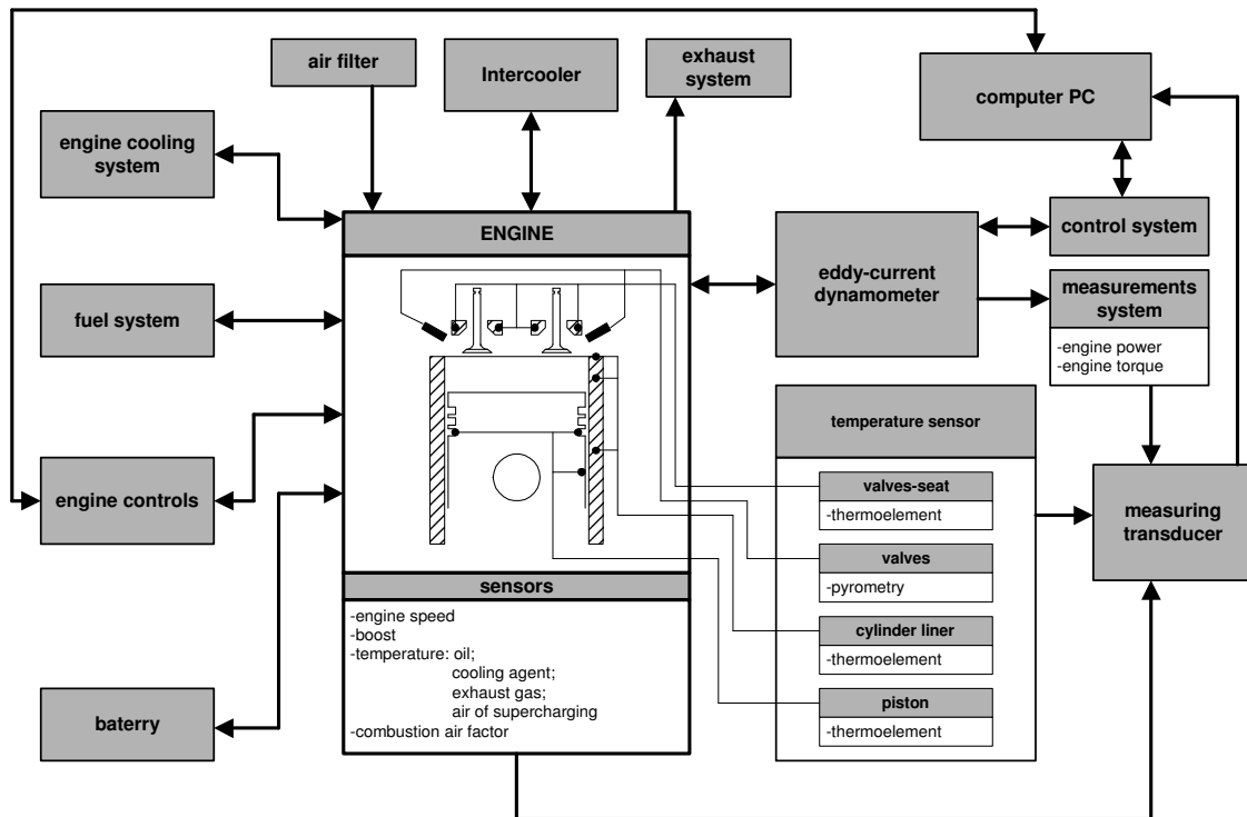
Fig. 3. Block diagram of measuring position
